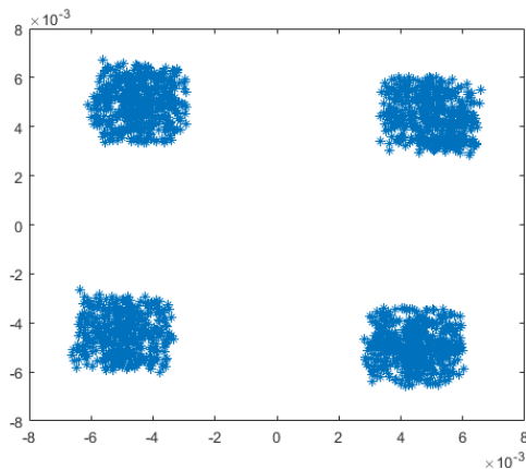
Recovered QPSK constellation at Rx2
